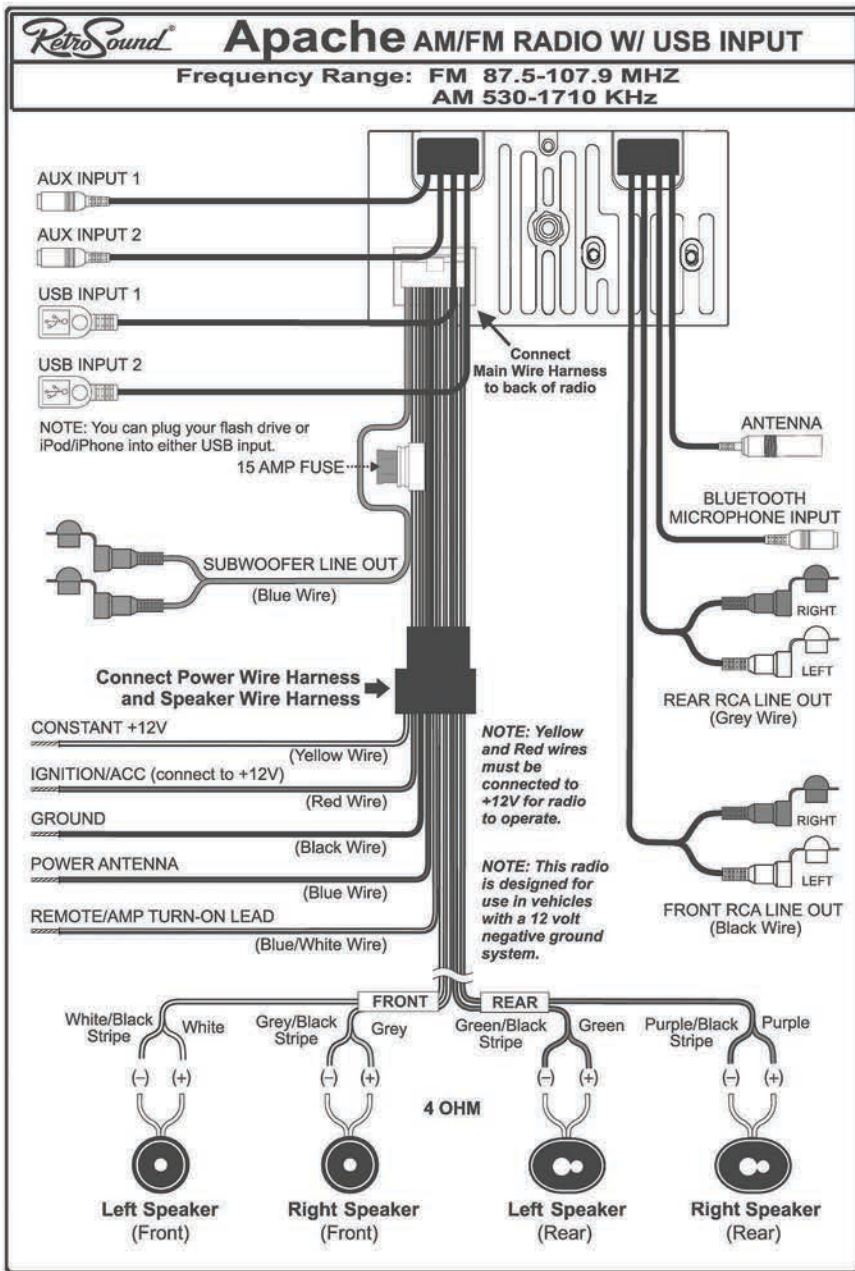
Figure 9 - Wiring Diagram
