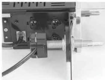
Figure 2 - Mount Shaft to Bracket
